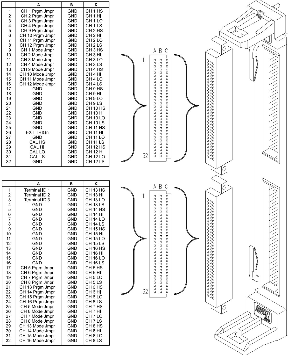
Figure 1-12 shows the connections at the terminal module connectors.
