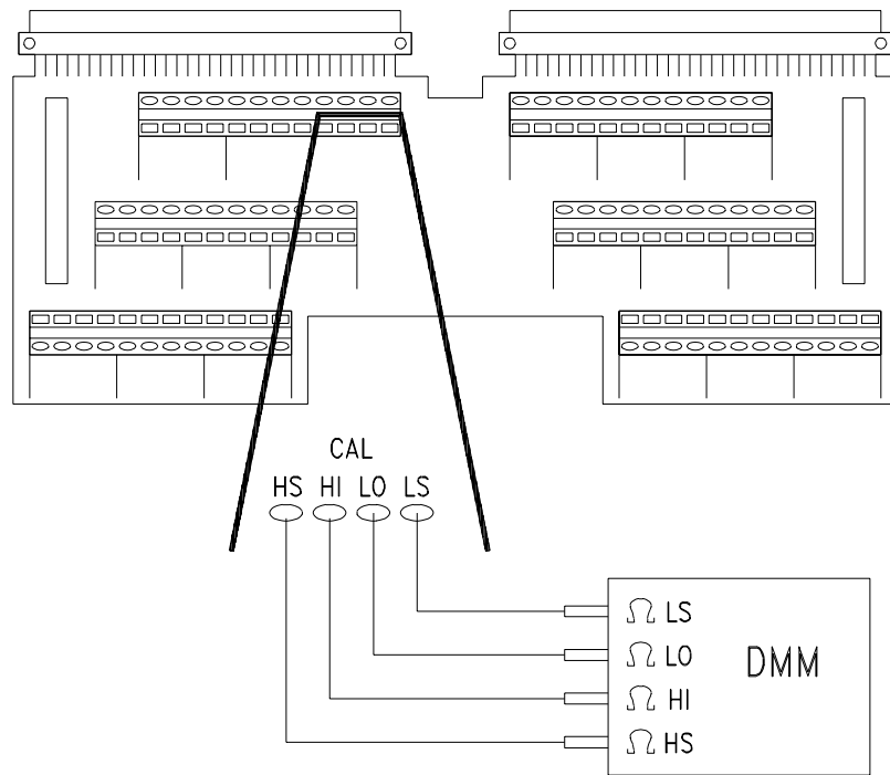
Figure 1-17. Calbus Connections
